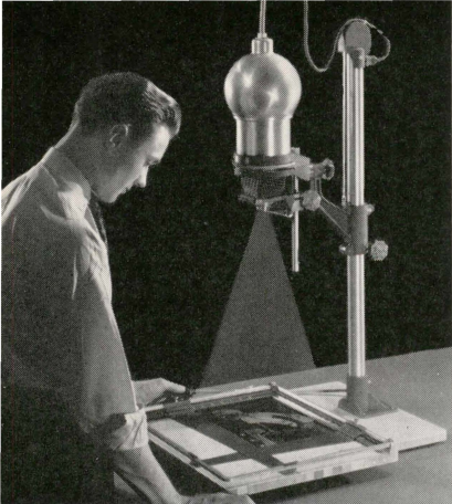
● At left: Kodak Precision Enlarger, A Assembly—one of the two enlarging assemblies. With available accessories, both this and the B Assembly can be converted for other photographic uses.
